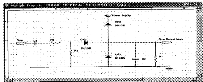
Figure 3: Phone detect circuit
